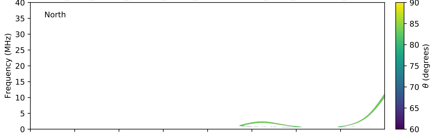
expres_juno_jupiter_europa_jrm09_lossc-wid1deg_3kev_20211102_v11.cdf
