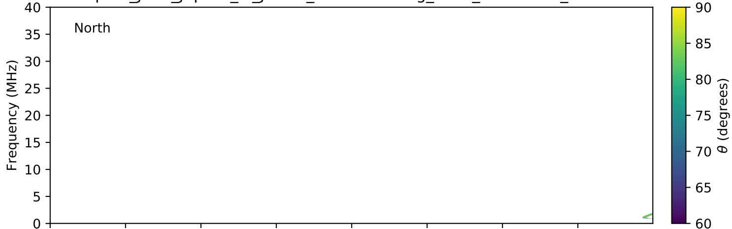
expres_juno_jupiter_io_jrm09_lossc-wid1deg_3kev_20211031_v11.cdf
