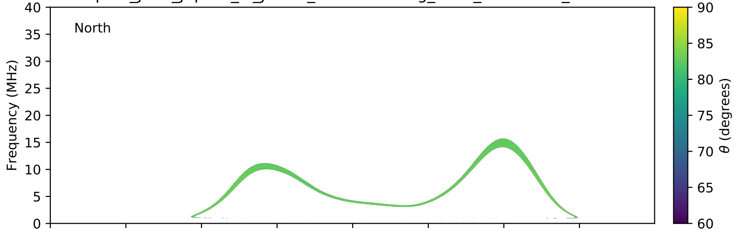
expres_juno_jupiter_io_jrm09_lossc-wid1deg_3kev_20211030_v11.cdf
