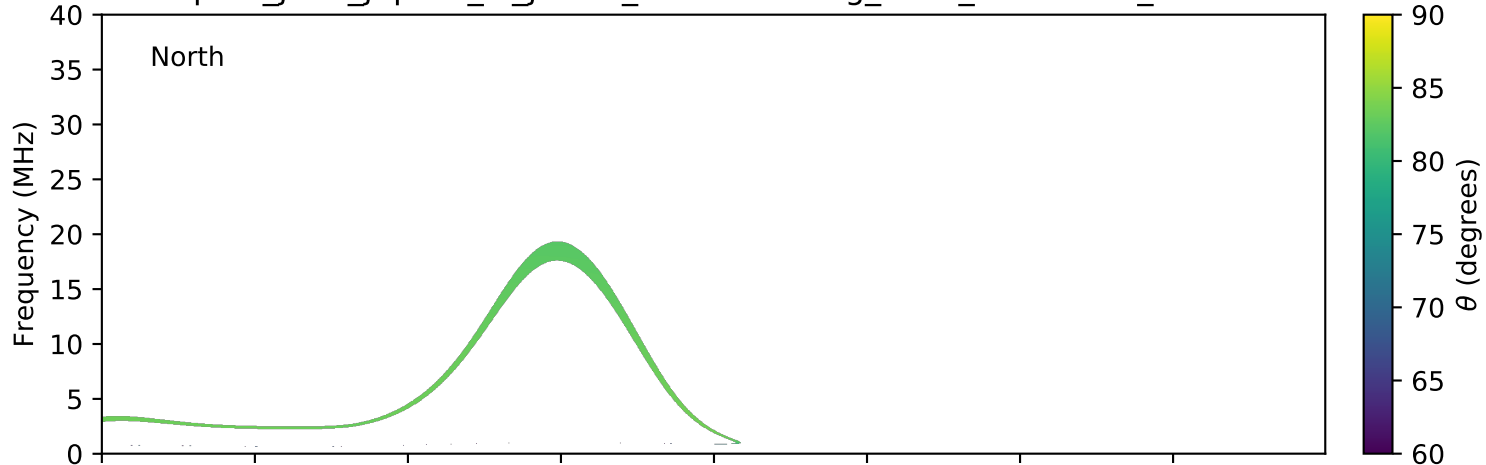
expres_juno_jupiter_io_jrm09_lossc-wid1deg_3kev_20211025_v11.cdf
