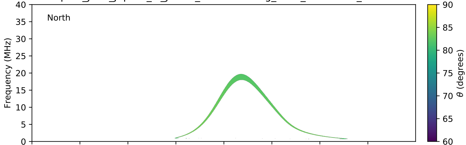
expres_juno_jupiter_io_jrm09_lossc-wid1deg_3kev_20211024_v11.cdf
