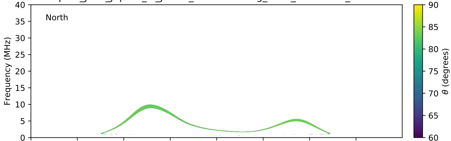
expres_juno_jupiter_io_jrm09_lossc-wid1deg_3kev_20211023_v11.cdf
