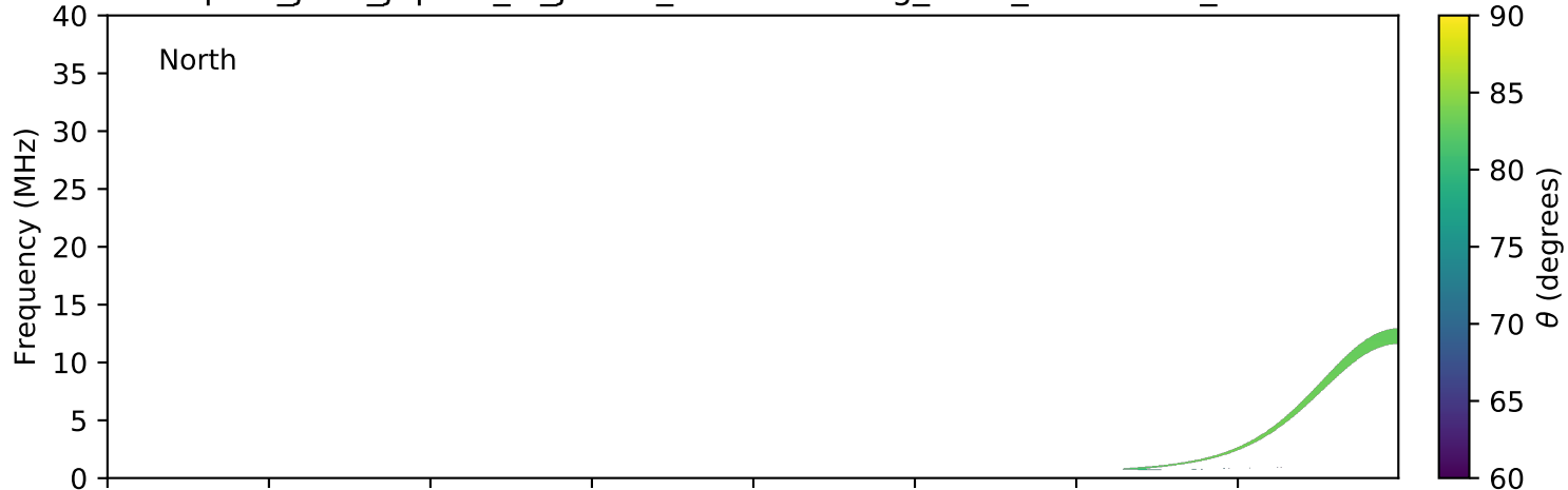
expres_juno_jupiter_io_jrm09_lossc-wid1deg_3kev_20211019_v11.cdf
