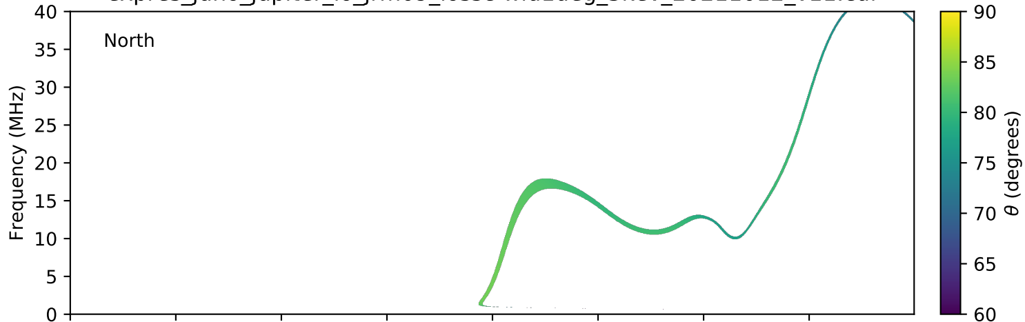
expres_juno_jupiter_io_jrm09_lossc-wid1deg_3kev_20211012_v11.cdf
