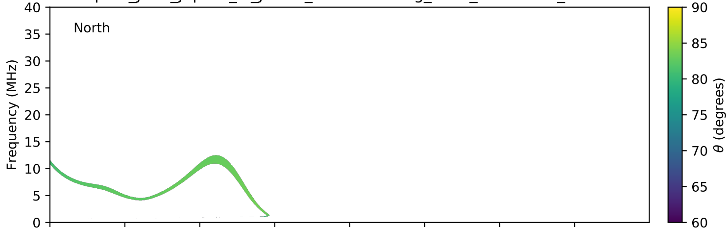
expres_juno_jupiter_io_jrm09_lossc-wid1deg_3kev_20211004_v11.cdf
