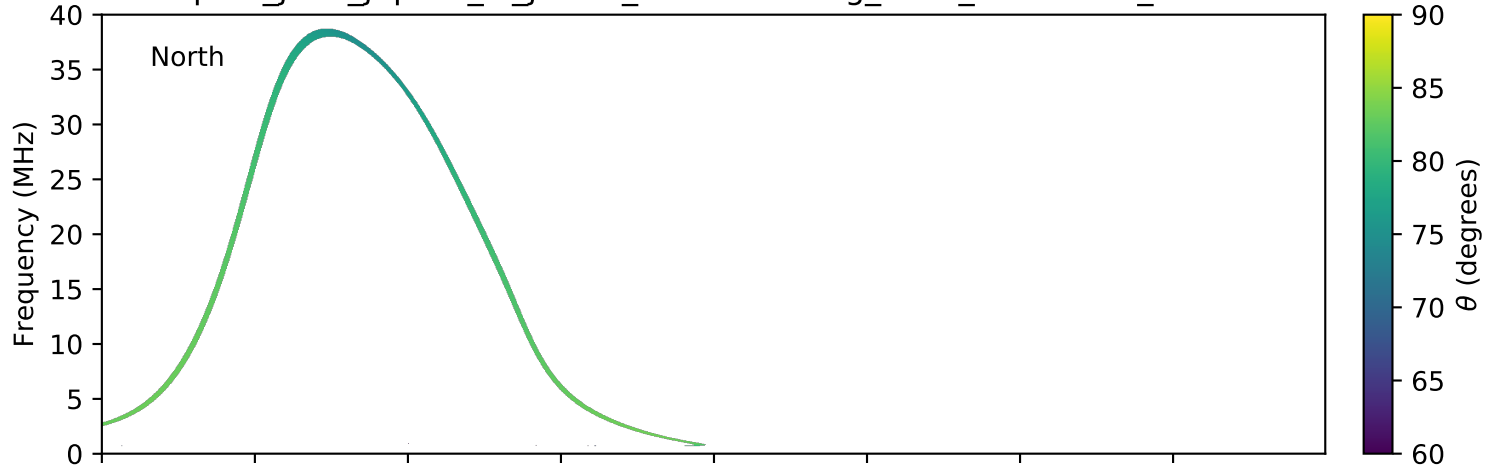
expres_juno_jupiter_io_jrm09_lossc-wid1deg_3kev_20211002_v11.cdf
