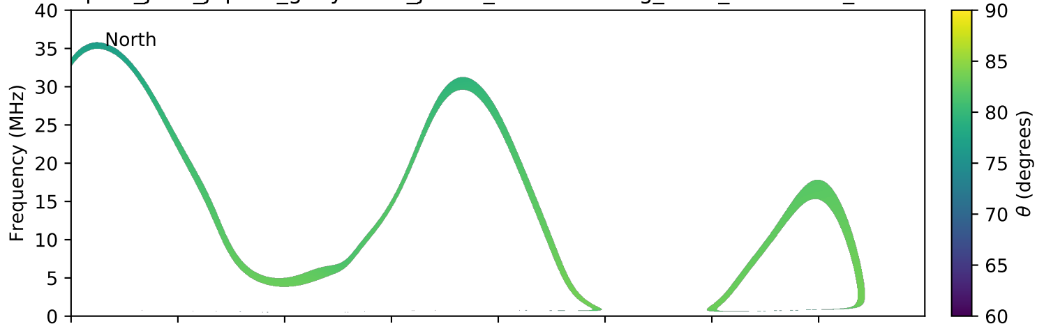
expres_juno_jupiter_ganymede_jrm09_lossc-wid1deg_3kev_20211015_v11.cdf
