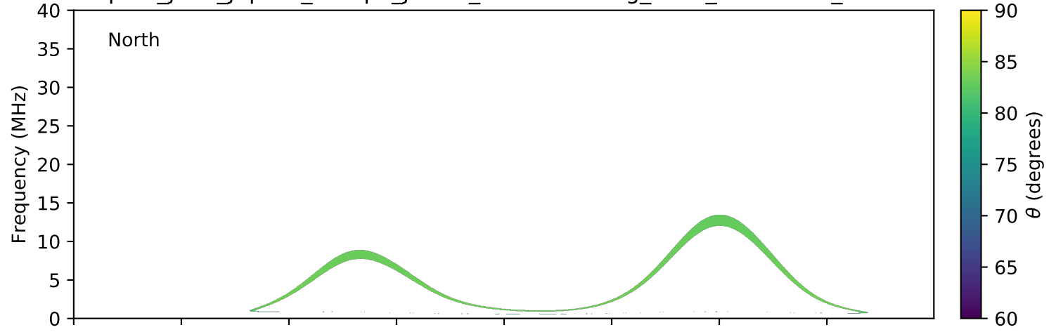
expres_juno_jupiter_europa_jrm09_lossc-wid1deg_3kev_20211030_v11.cdf
