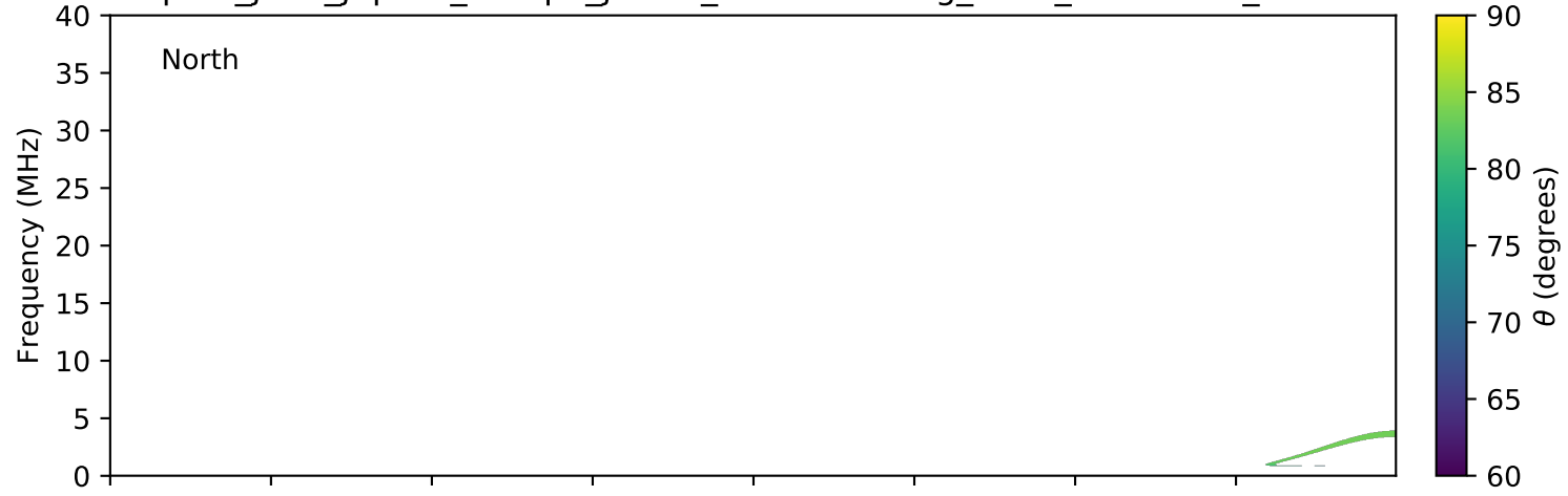
expres_juno_jupiter_europa_jrm09_lossc-wid1deg_3kev_20211019_v11.cdf
