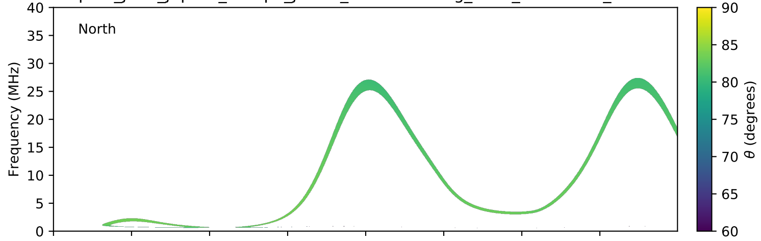
expres_juno_jupiter_europa_jrm09_lossc-wid1deg_3kev_20211005_v11.cdf
