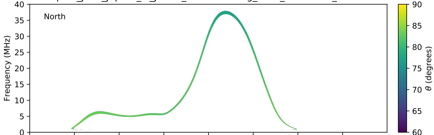
expres_juno_jupiter_io_jrm09_lossc-wid1deg_3kev_20210930_v11.cdf
