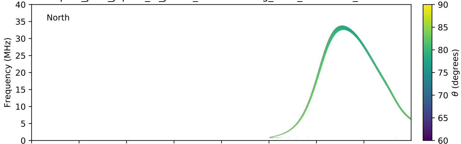
expres_juno_jupiter_io_jrm09_lossc-wid1deg_3kev_20210926_v11.cdf
