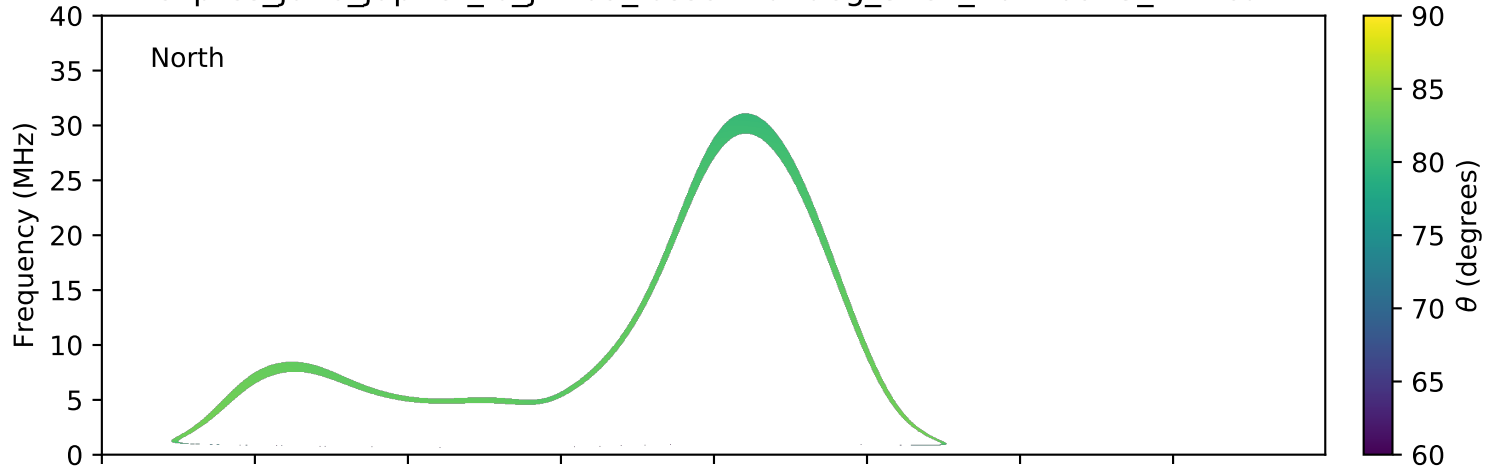
expres_juno_jupiter_io_jrm09_lossc-wid1deg_3kev_20210923_v11.cdf
