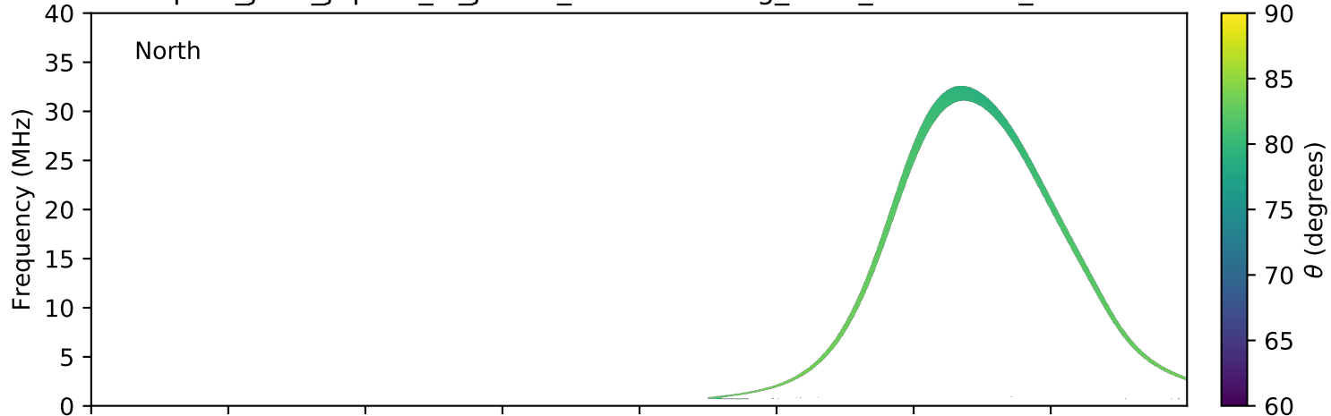
expres_juno_jupiter_io_jrm09_lossc-wid1deg_3kev_20210919_v11.cdf
