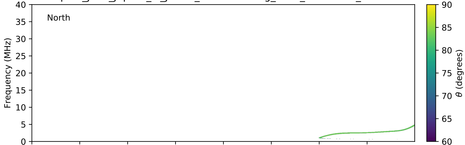
expres_juno_jupiter_io_jrm09_lossc-wid1deg_3kev_20210917_v11.cdf
