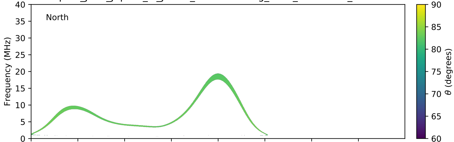
expres_juno_jupiter_io_jrm09_lossc-wid1deg_3kev_20210916_v11.cdf
