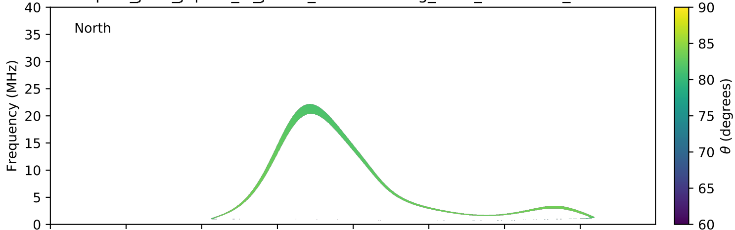
expres_juno_jupiter_io_jrm09_lossc-wid1deg_3kev_20210914_v11.cdf
