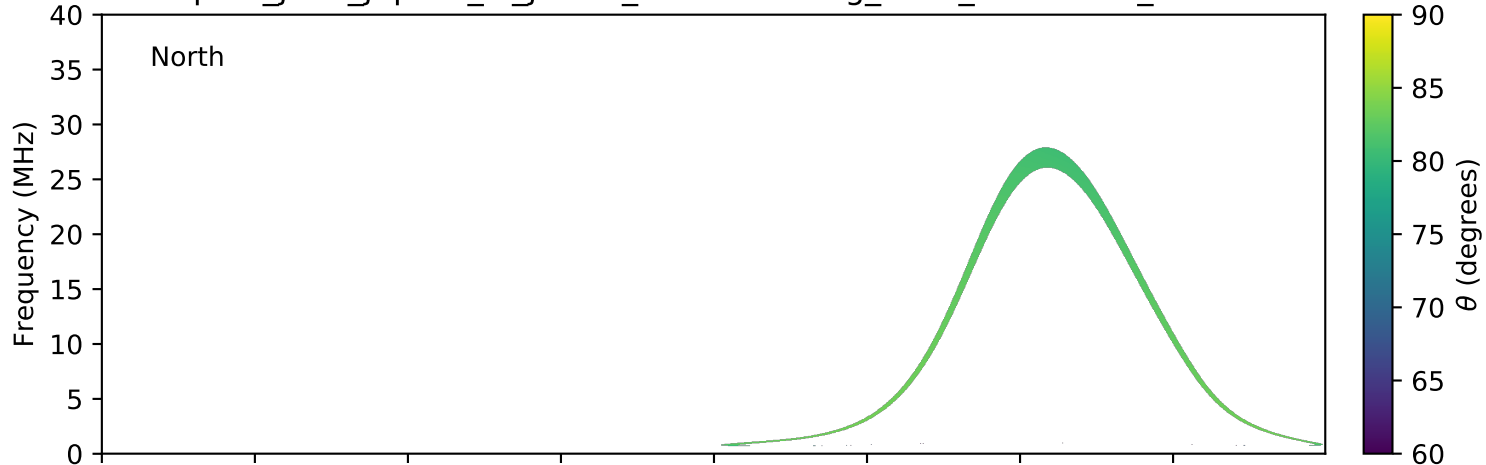
expres_juno_jupiter_io_jrm09_lossc-wid1deg_3kev_20210912_v11.cdf
