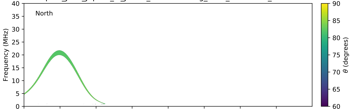
expres_juno_jupiter_io_jrm09_lossc-wid1deg_3kev_20210911_v11.cdf
