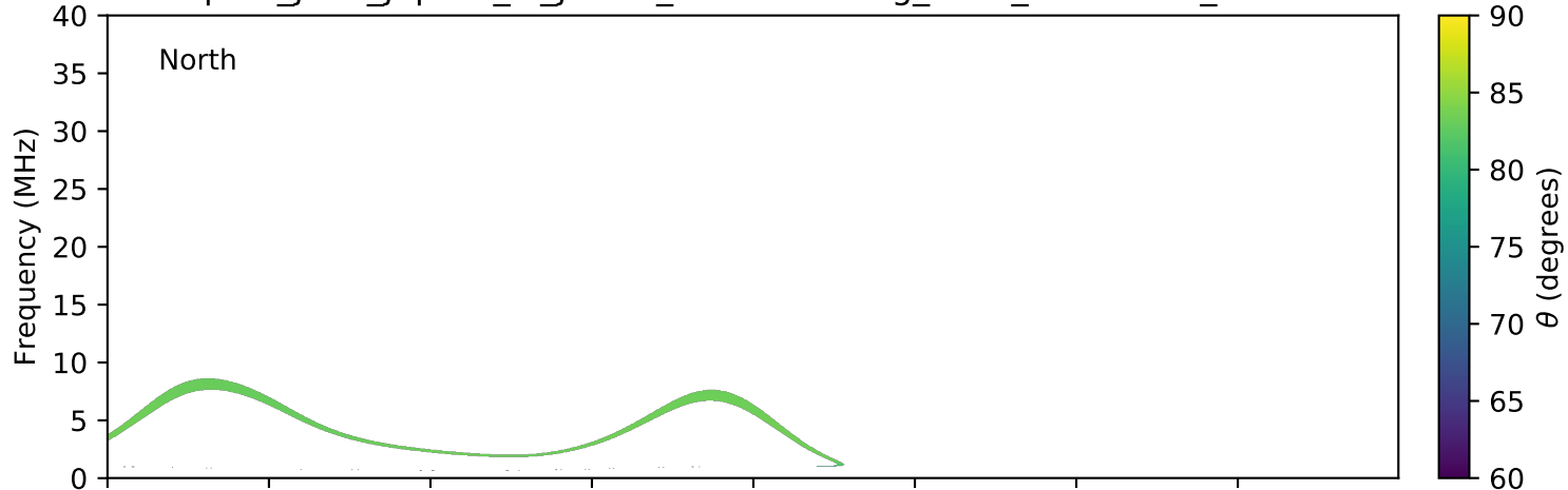
expres_juno_jupiter_io_jrm09_lossc-wid1deg_3kev_20210909_v11.cdf
