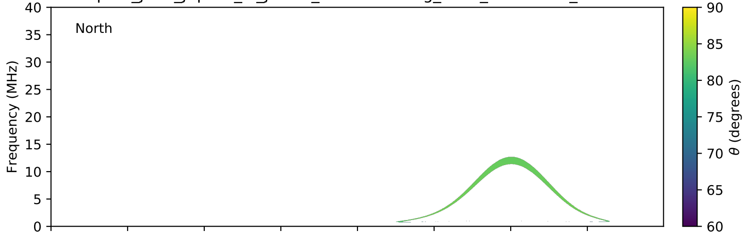
expres_juno_jupiter_io_jrm09_lossc-wid1deg_3kev_20210905_v11.cdf
