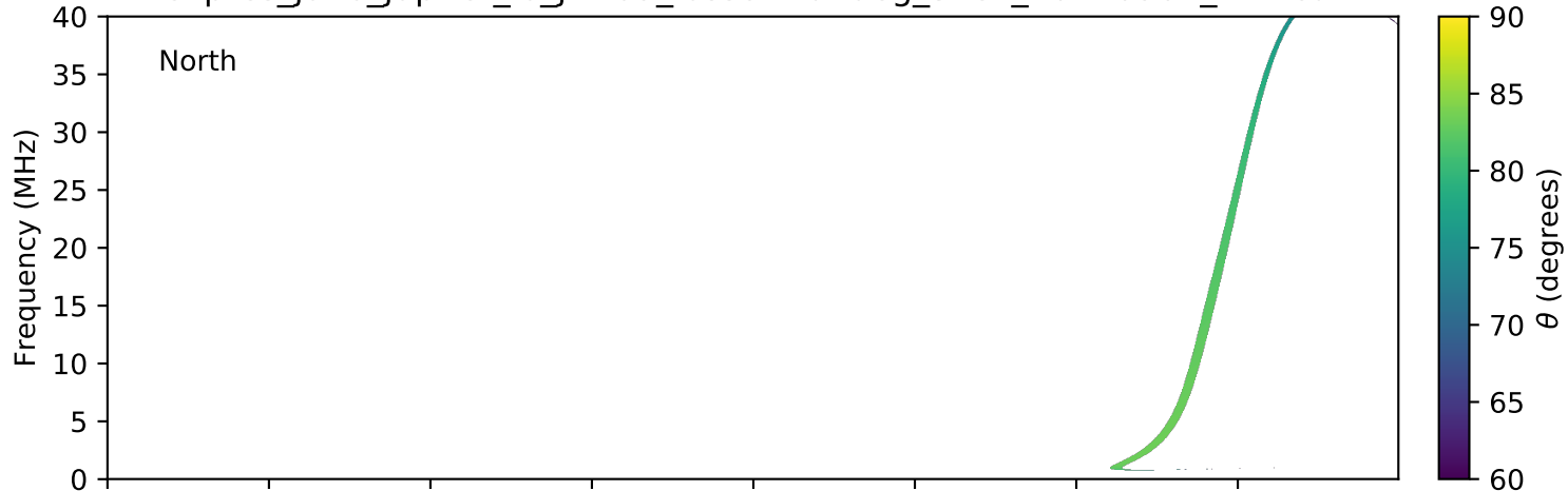
expres_juno_jupiter_io_jrm09_lossc-wid1deg_3kev_20210901_v11.cdf
