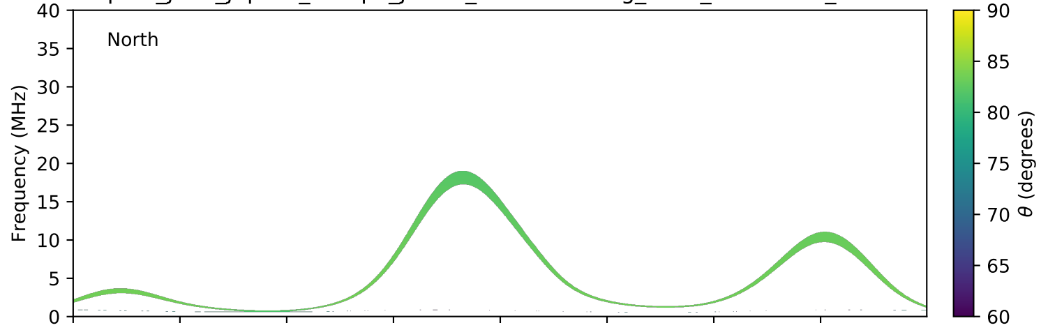
expres_juno_jupiter_europa_jrm09_lossc-wid1deg_3kev_20210921_v11.cdf
