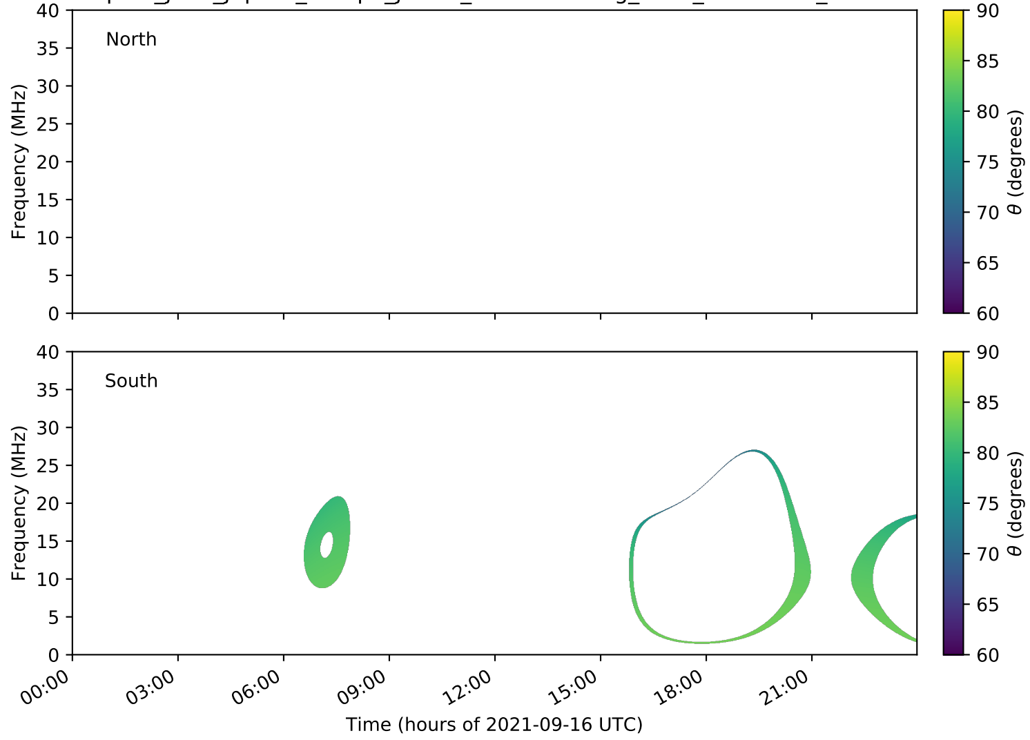
expres_juno_jupiter_europa_jrm09_lossc-wid1deg_3kev_20210916_v11.cdf
