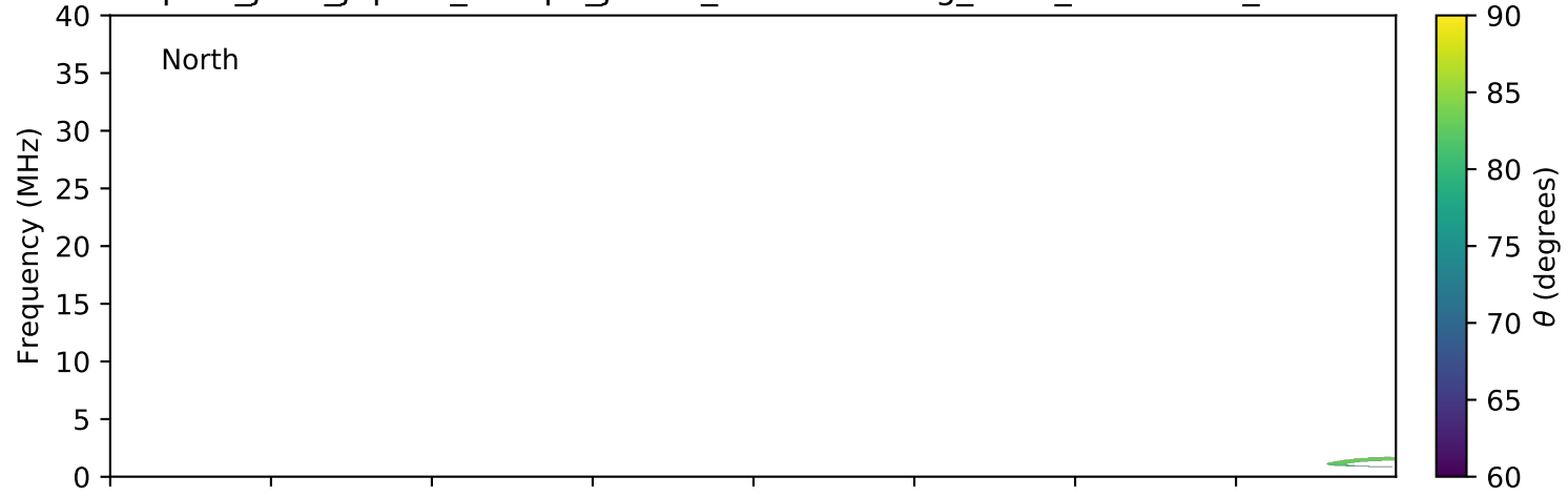
expres_juno_jupiter_europa_jrm09_lossc-wid1deg_3kev_20210906_v11.cdf
