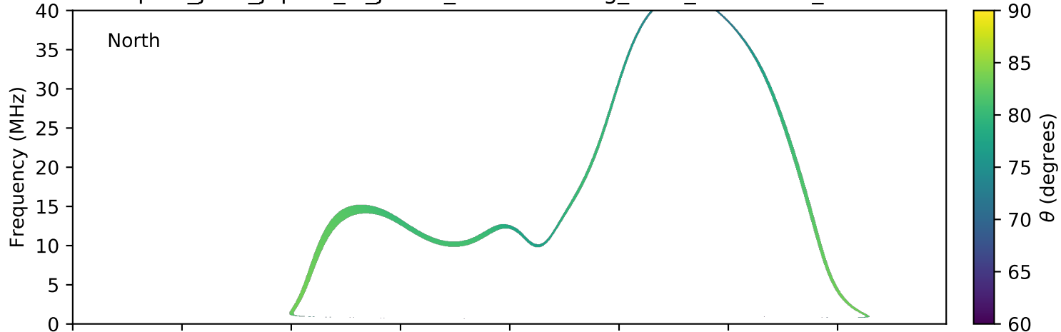
expres_juno_jupiter_io_jrm09_lossc-wid1deg_3kev_20210829_v11.cdf
