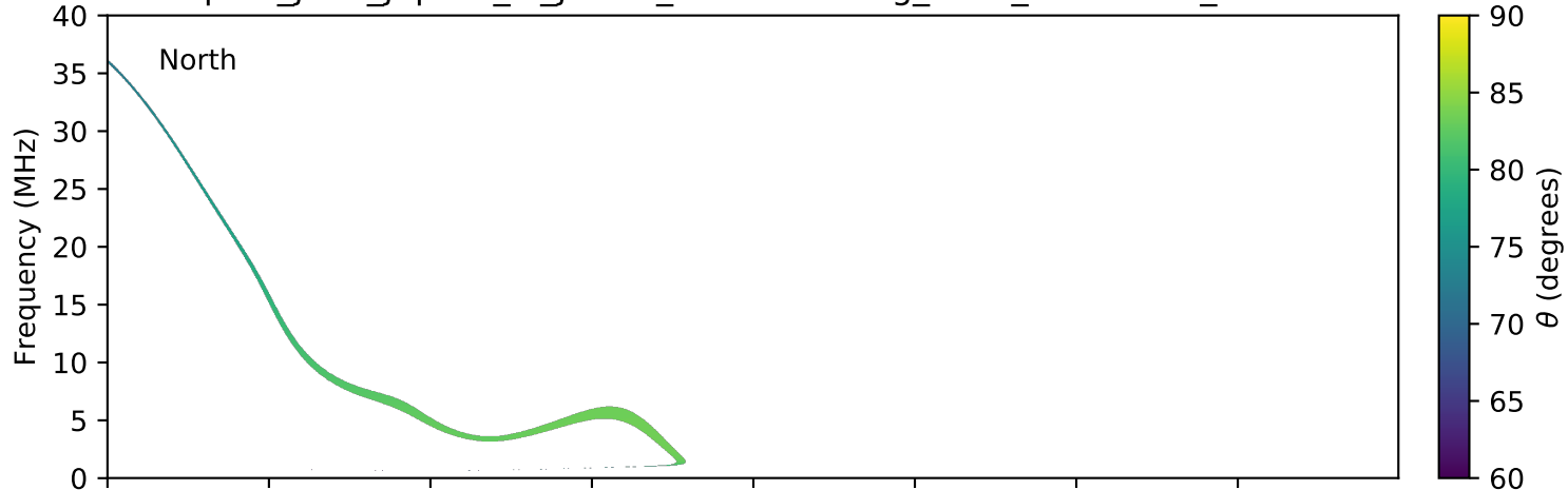
expres_juno_jupiter_io_jrm09_lossc-wid1deg_3kev_20210826_v11.cdf
