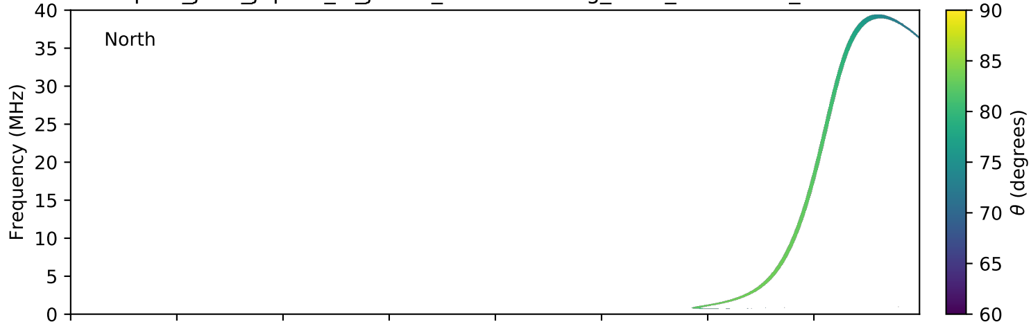
expres_juno_jupiter_io_jrm09_lossc-wid1deg_3kev_20210825_v11.cdf
