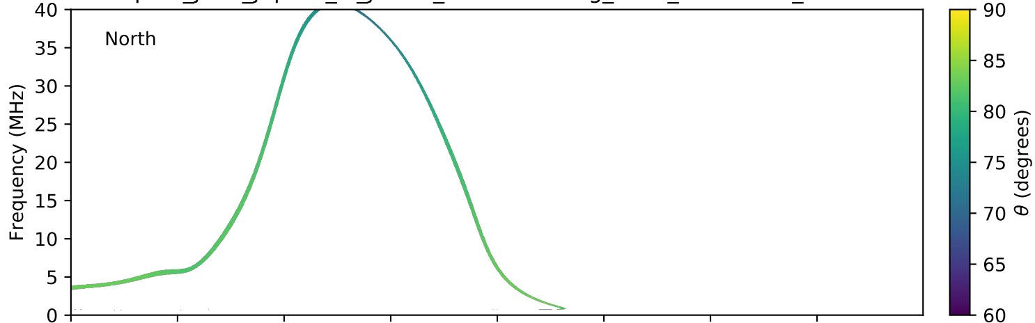
expres_juno_jupiter_io_jrm09_lossc-wid1deg_3kev_20210824_v11.cdf
