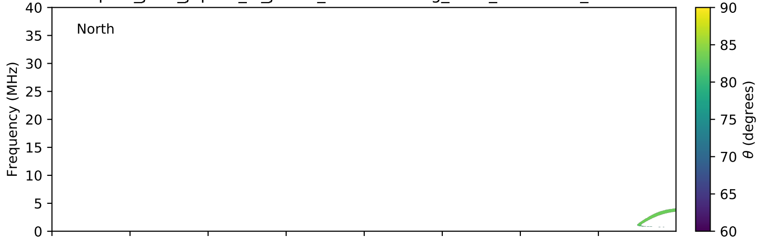
expres_juno_jupiter_io_jrm09_lossc-wid1deg_3kev_20210823_v11.cdf
