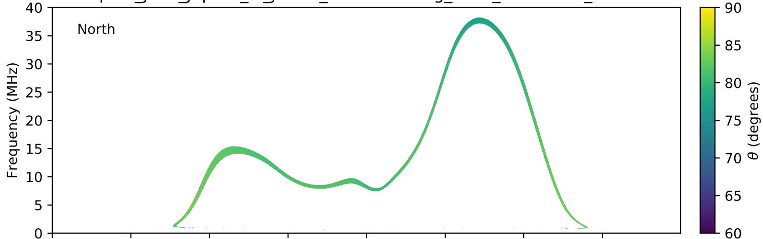
expres_juno_jupiter_io_jrm09_lossc-wid1deg_3kev_20210822_v11.cdf
