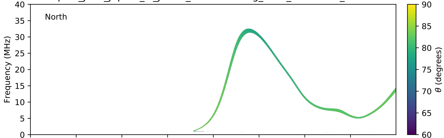
expres_juno_jupiter_io_jrm09_lossc-wid1deg_3kev_20210820_v11.cdf
