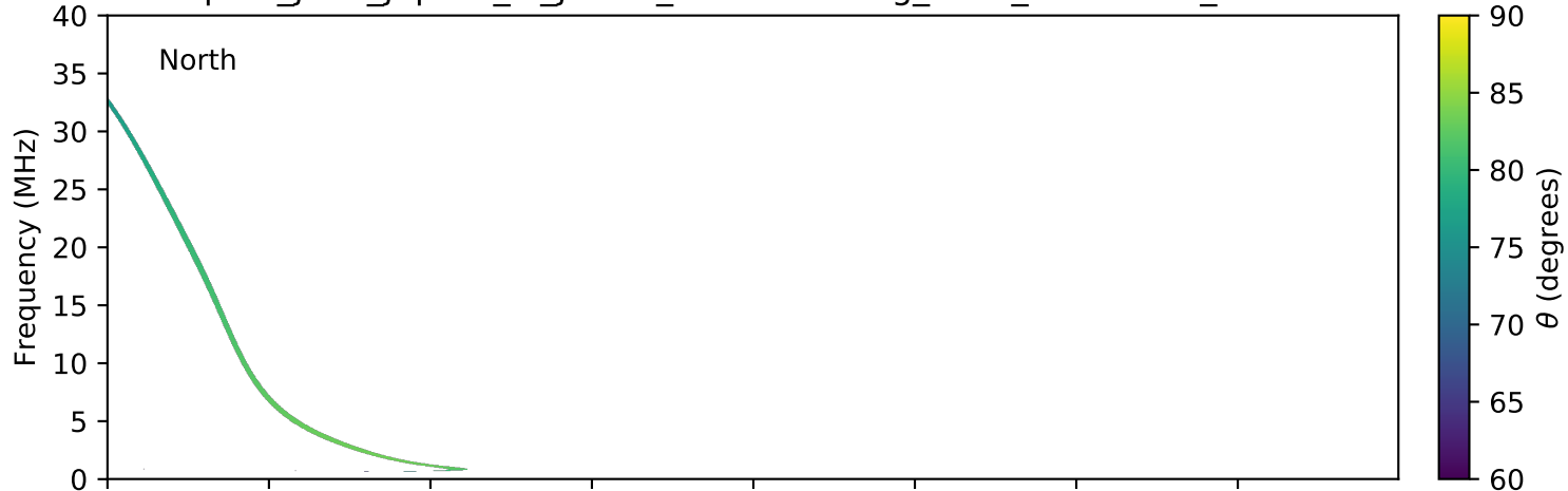
expres_juno_jupiter_io_jrm09_lossc-wid1deg_3kev_20210819_v11.cdf
