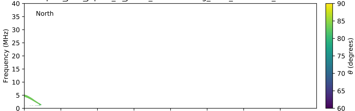
expres_juno_jupiter_io_jrm09_lossc-wid1deg_3kev_20210814_v11.cdf
