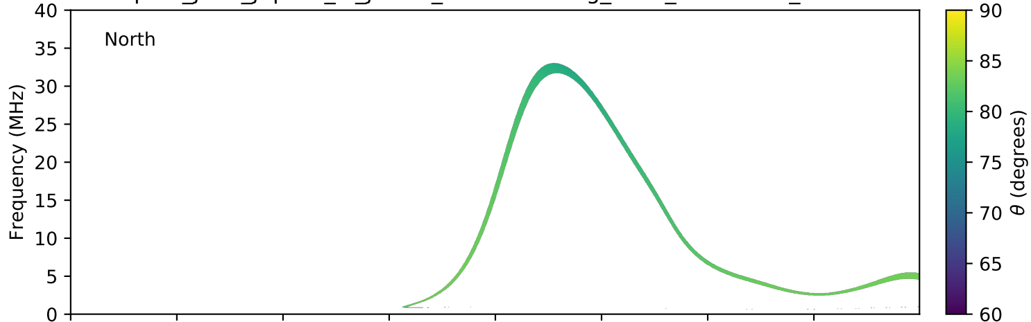
expres_juno_jupiter_io_jrm09_lossc-wid1deg_3kev_20210813_v11.cdf
