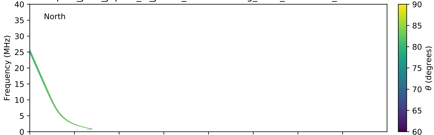
expres_juno_jupiter_io_jrm09_lossc-wid1deg_3kev_20210812_v11.cdf
