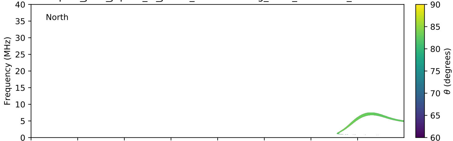
expres_juno_jupiter_io_jrm09_lossc-wid1deg_3kev_20210809_v11.cdf
