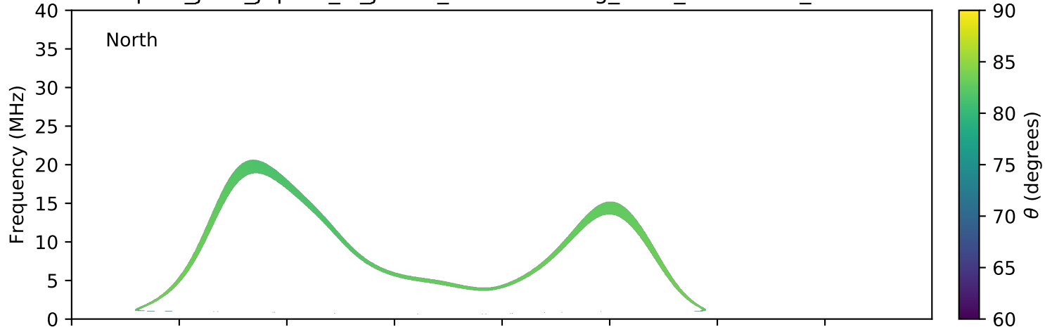
expres_juno_jupiter_io_jrm09_lossc-wid1deg_3kev_20210808_v11.cdf
