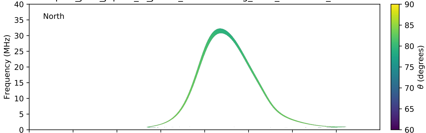
expres_juno_jupiter_io_jrm09_lossc-wid1deg_3kev_20210806_v11.cdf
