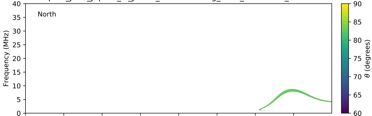
expres_juno_jupiter_io_jrm09_lossc-wid1deg_3kev_20210802_v11.cdf
