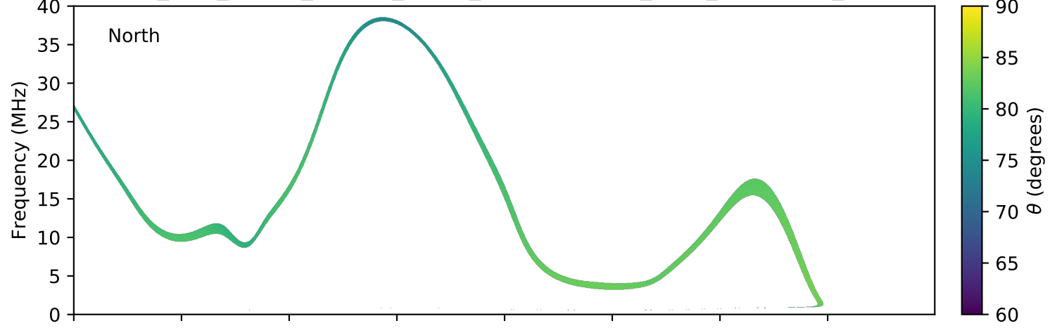
expres_juno_jupiter_europa_jrm09_lossc-wid1deg_3kev_20210831_v11.cdf
