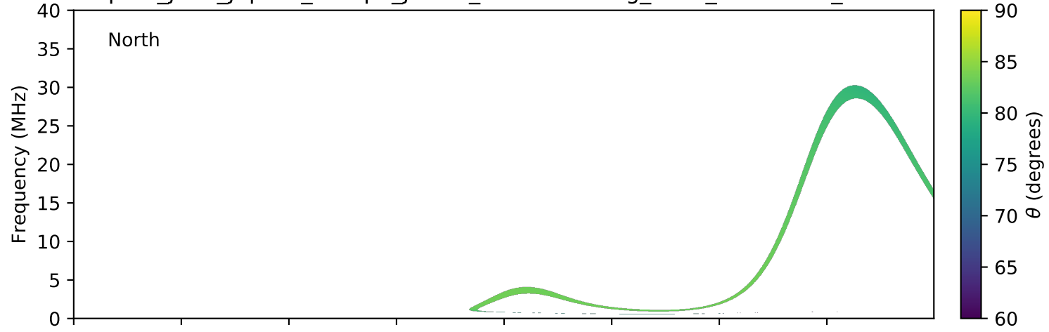
expres_juno_jupiter_europa_jrm09_lossc-wid1deg_3kev_20210823_v11.cdf
