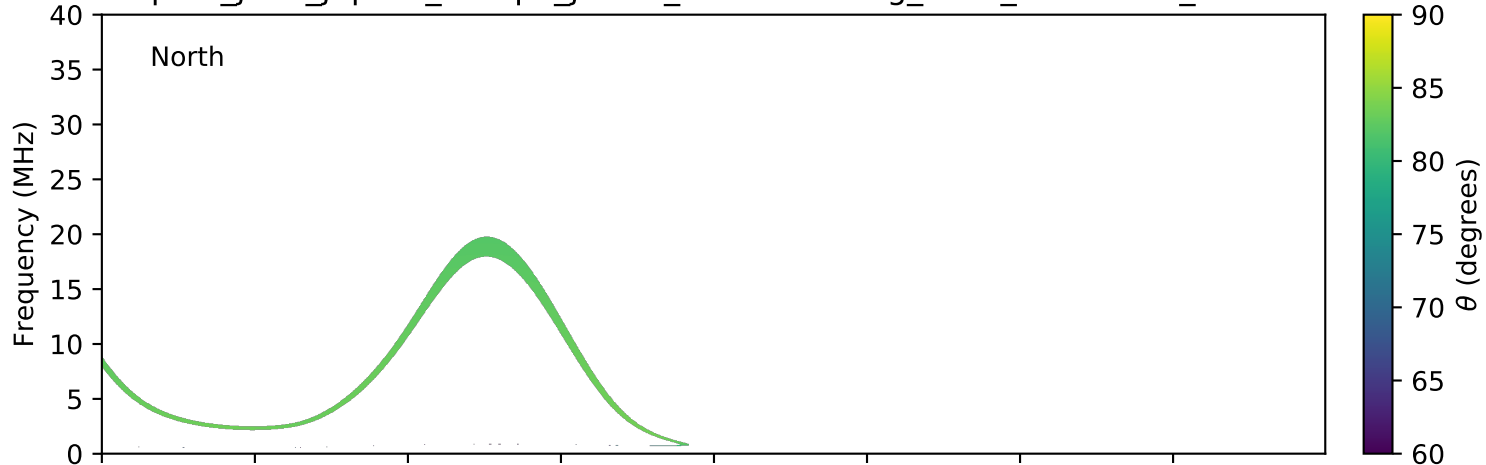
expres_juno_jupiter_europa_jrm09_lossc-wid1deg_3kev_20210817_v11.cdf
