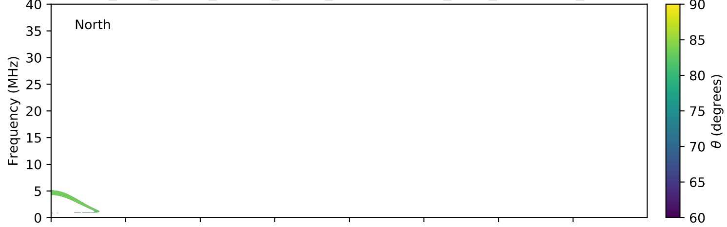
expres_juno_jupiter_europa_jrm09_lossc-wid1deg_3kev_20210814_v11.cdf
