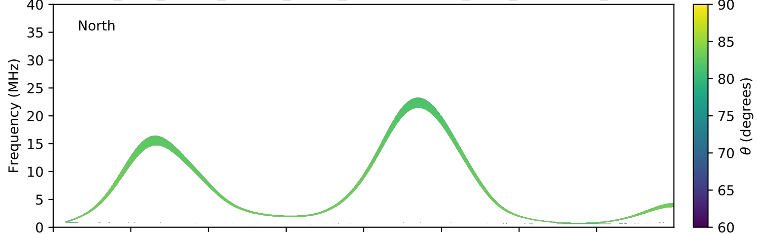
expres_juno_jupiter_europa_jrm09_lossc-wid1deg_3kev_20210813_v11.cdf
