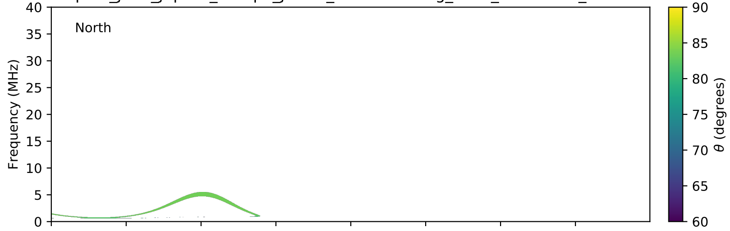
expres_juno_jupiter_europa_jrm09_lossc-wid1deg_3kev_20210803_v11.cdf
